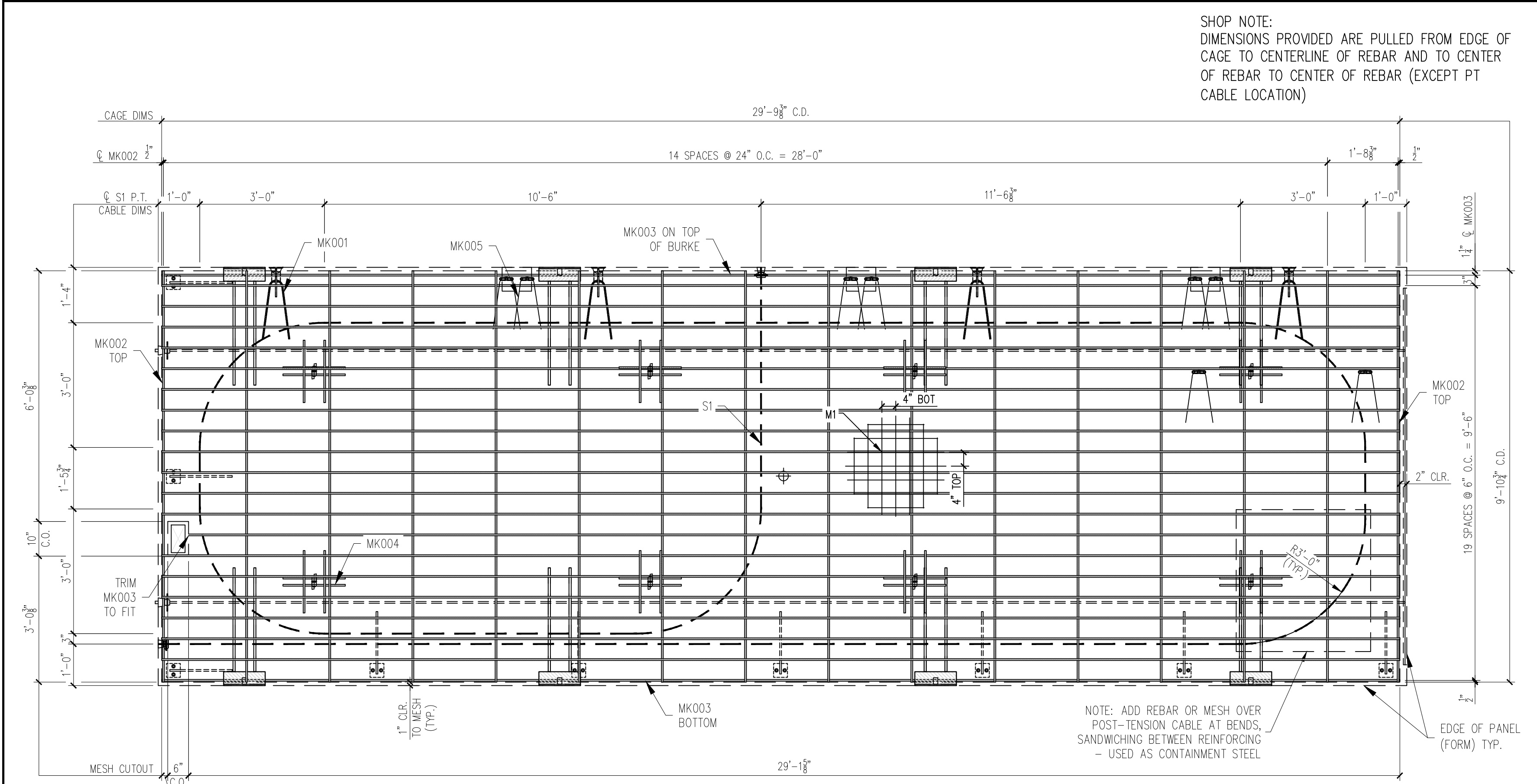
FLOOR REINFORCING VIEW SCALE: 1/2" = 1'-0"
