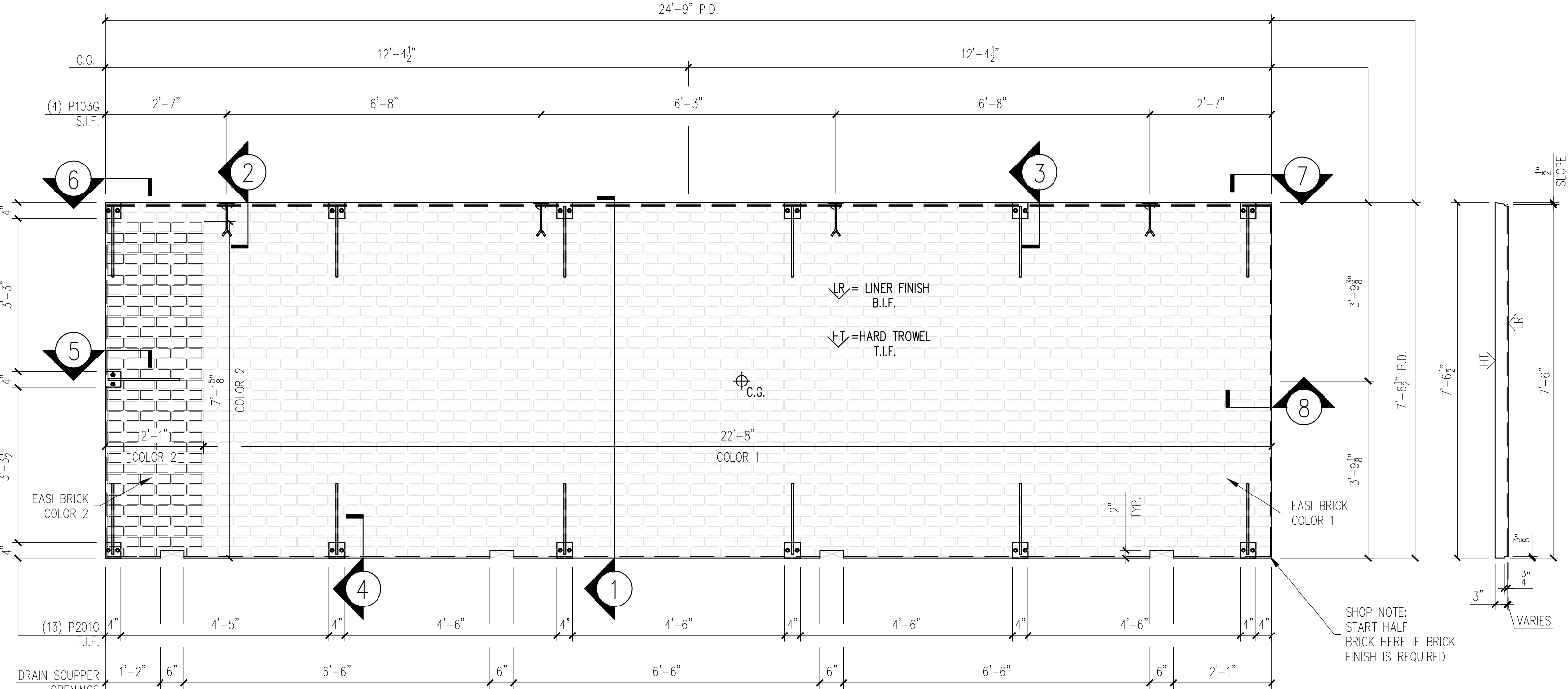
FORM VIEW SCALE: 1/2" = 1'-0"
