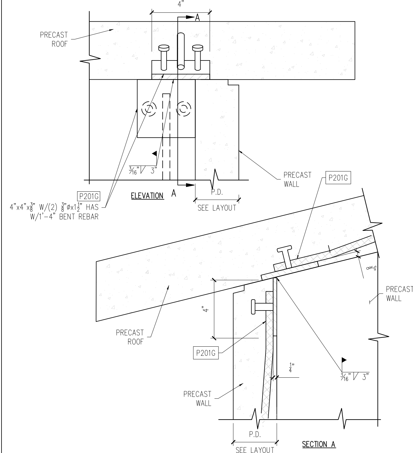
WALL TO ROOF CONNECTION (MID-SPAN)
