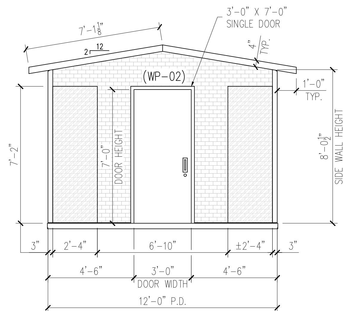
WEST ELEVATION
