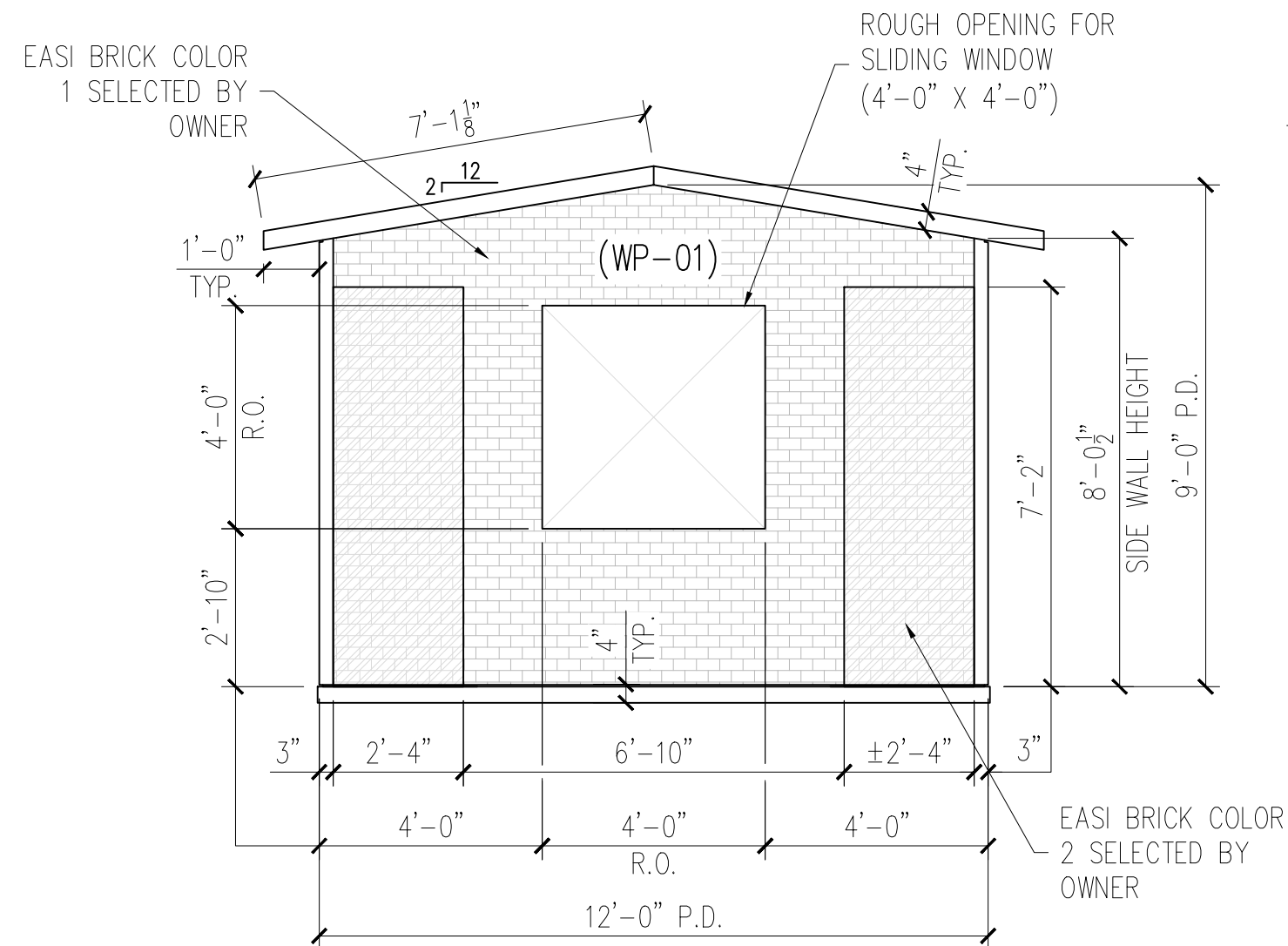
EAST ELEVATION
