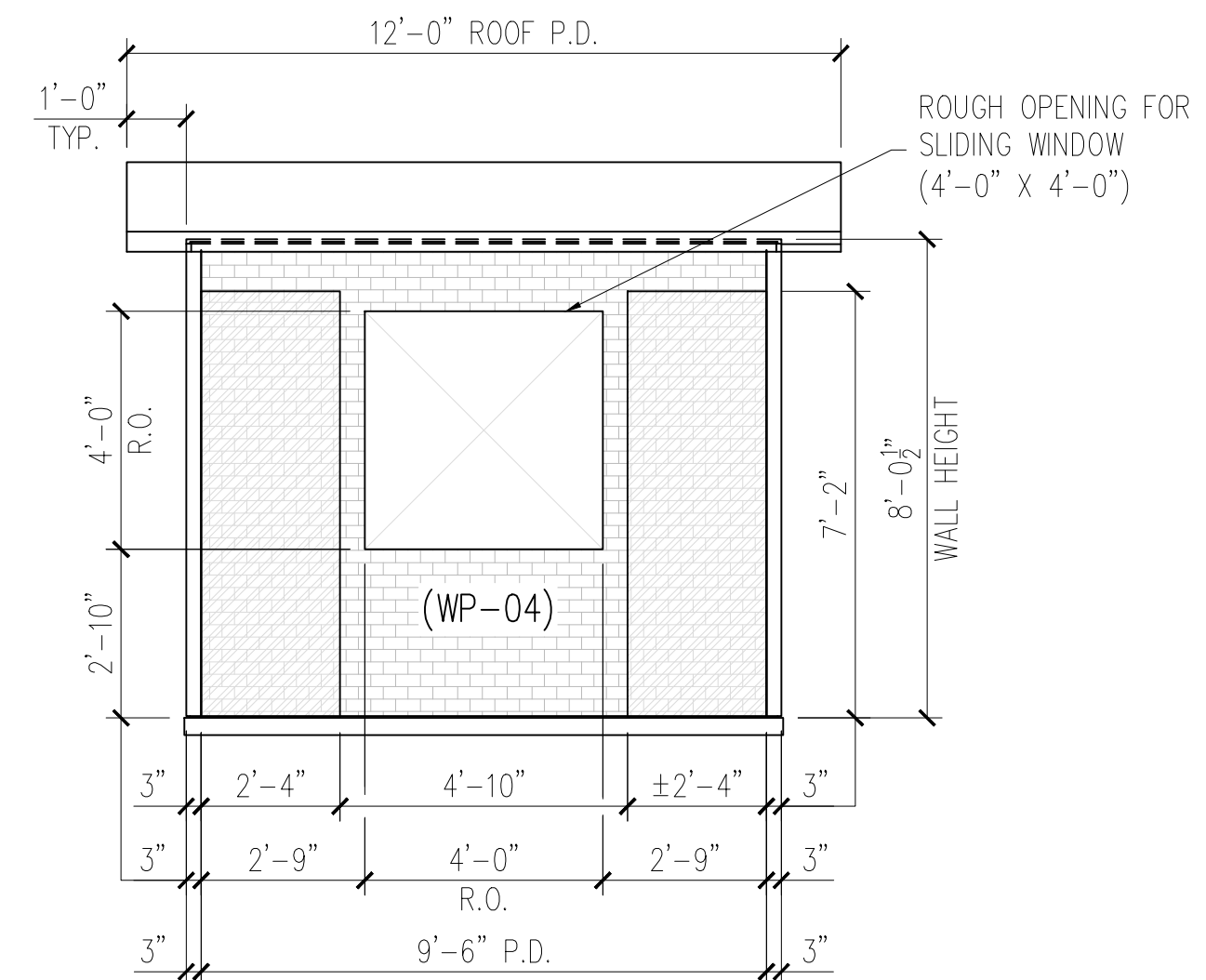
SOUTH ELEVATION
