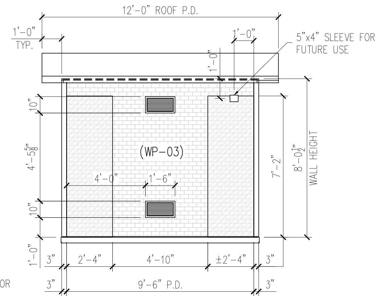
NORTH ELEVATION
