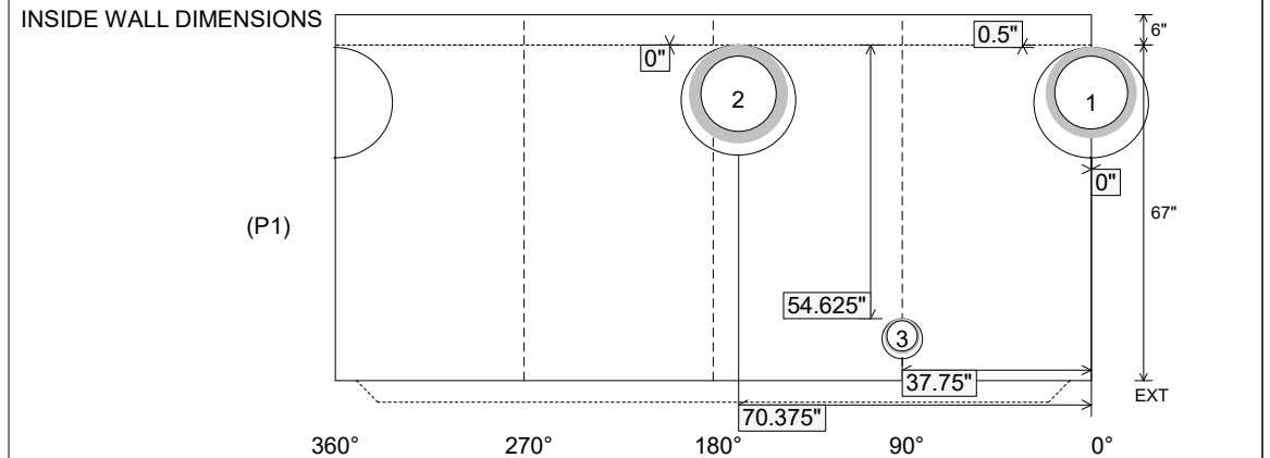
INSIDE WALL DIMENSIONS
