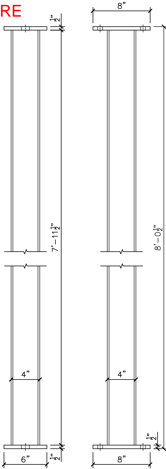
SIDE VIEW
