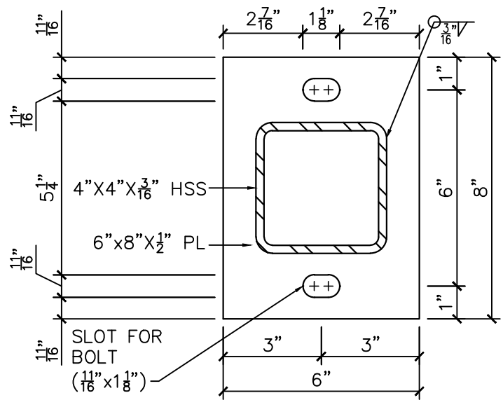
BASE PLATE
