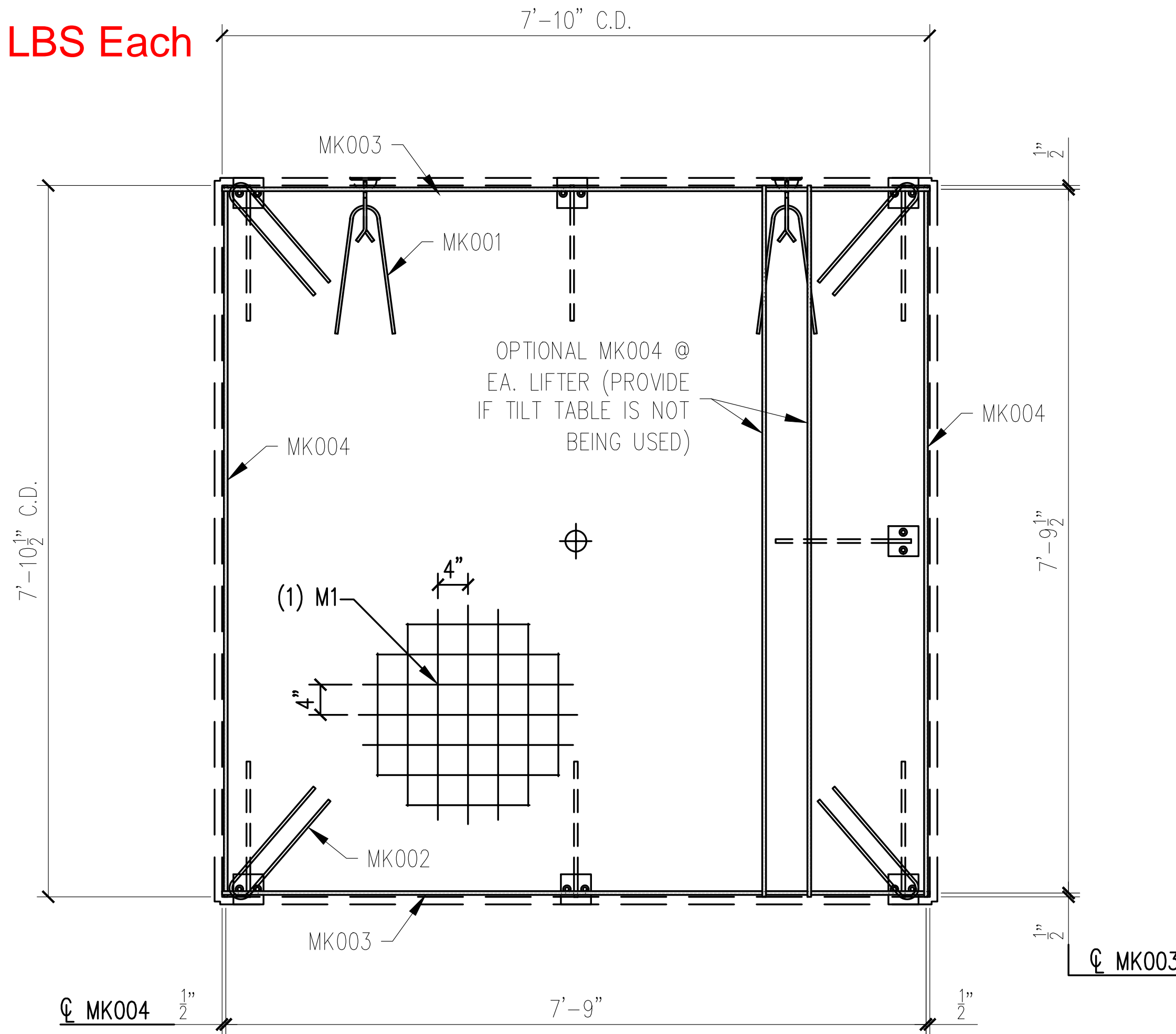
WALL REINFORCING VIEW SCALE: 1/2" = 1'-0"
