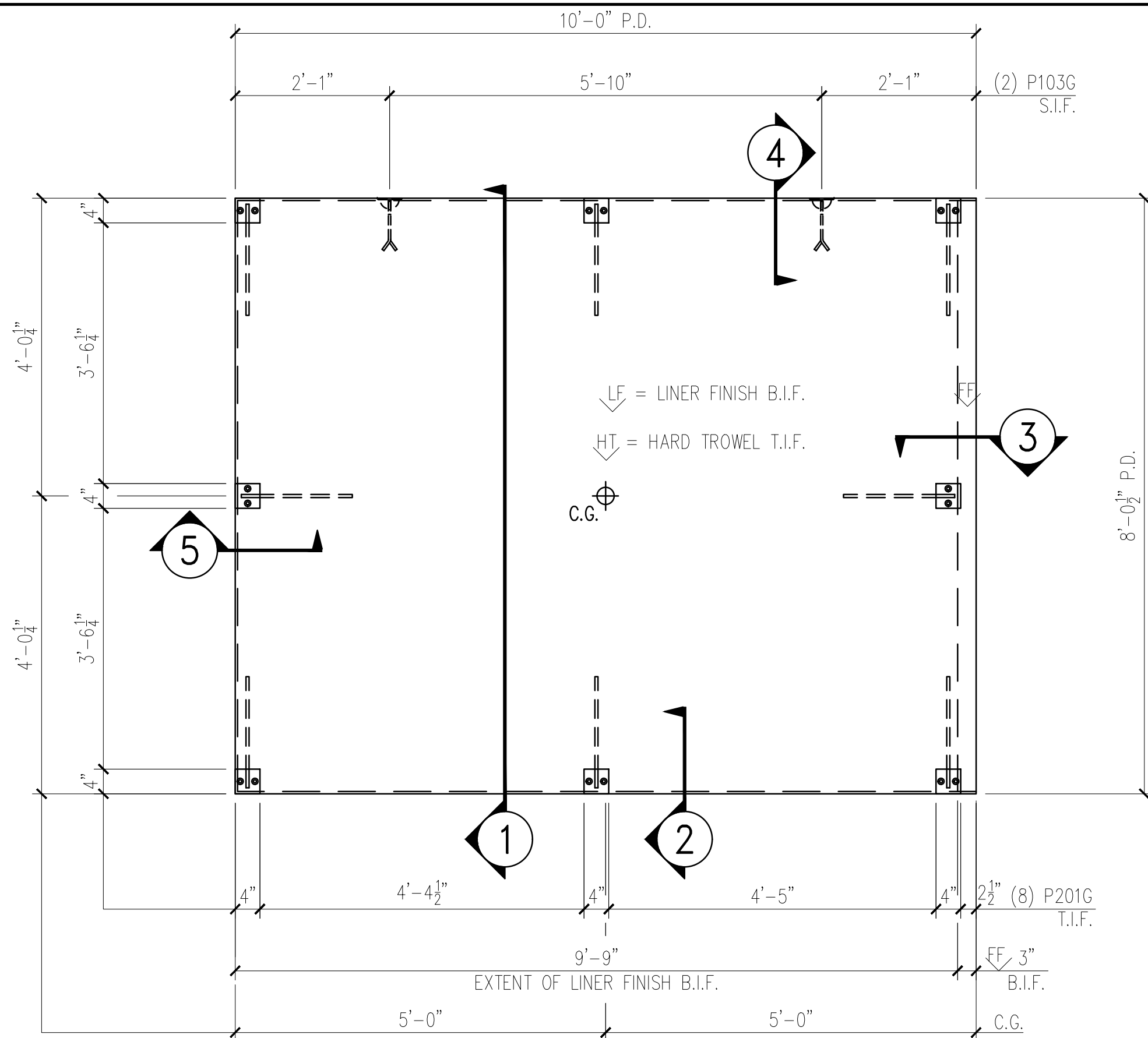
WALL FORM VIEW SCALE: 1/2" = 1'-0"
