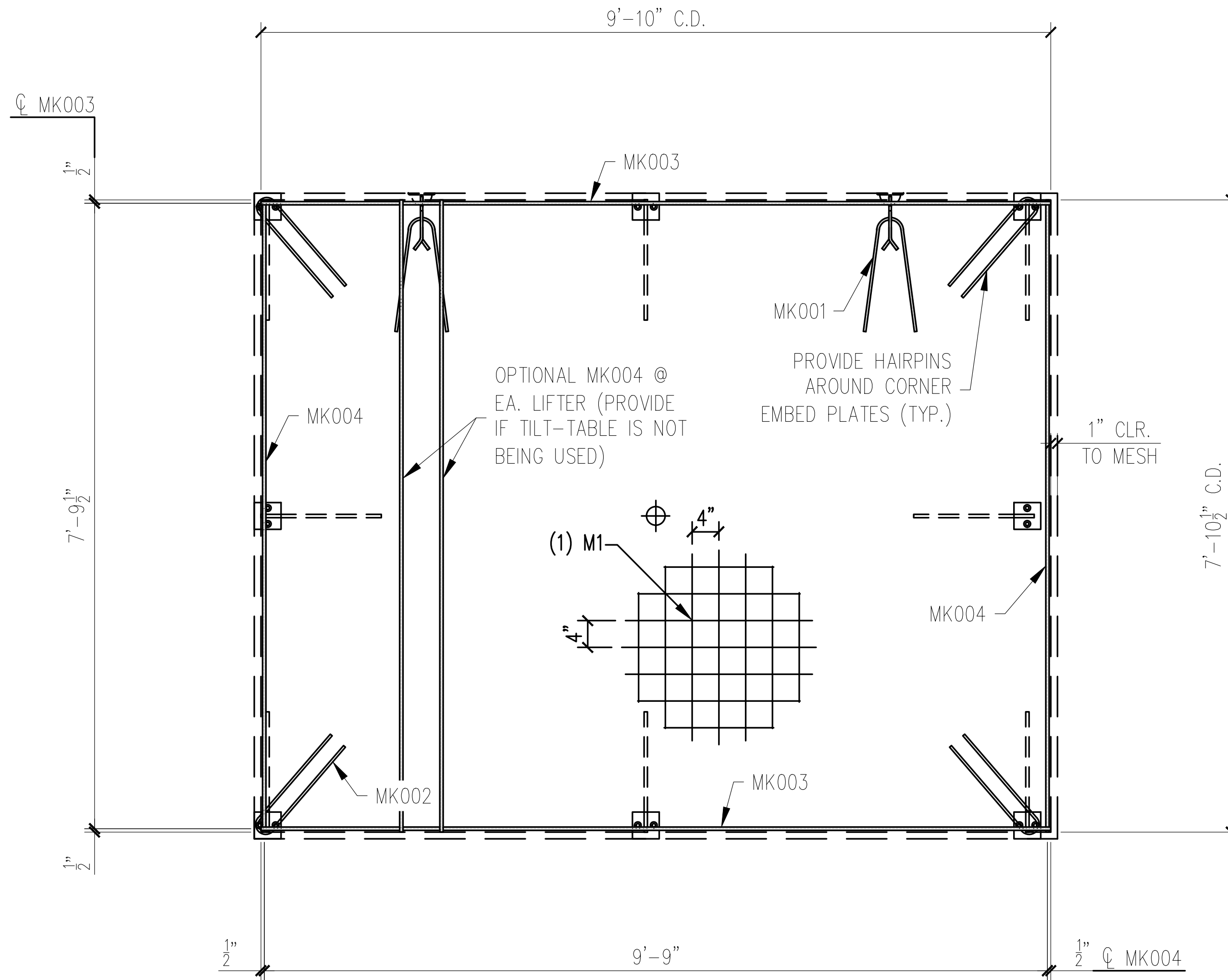
WALL REINFORCING VIEW
