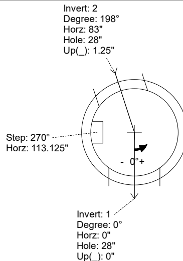
UPSIDE-DOWN VIEW (int. dimensions)
