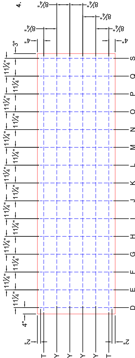
MAT REBAR LAYOUT
