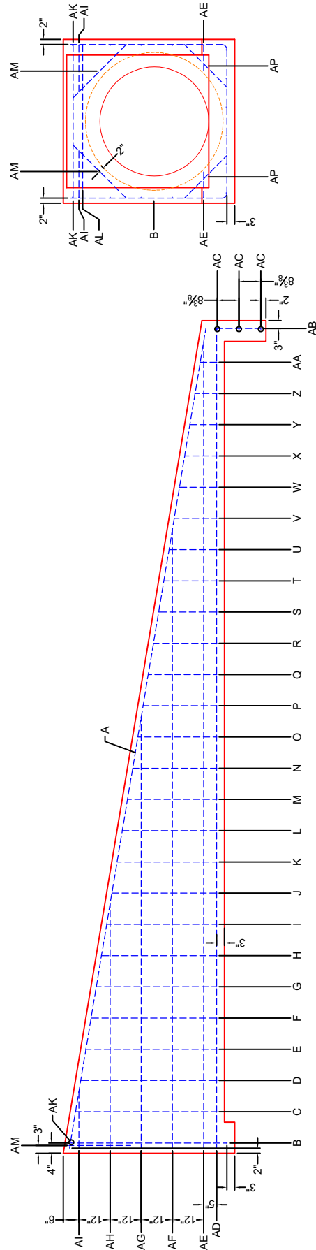
BACK WALL REBAR LAYOUT
