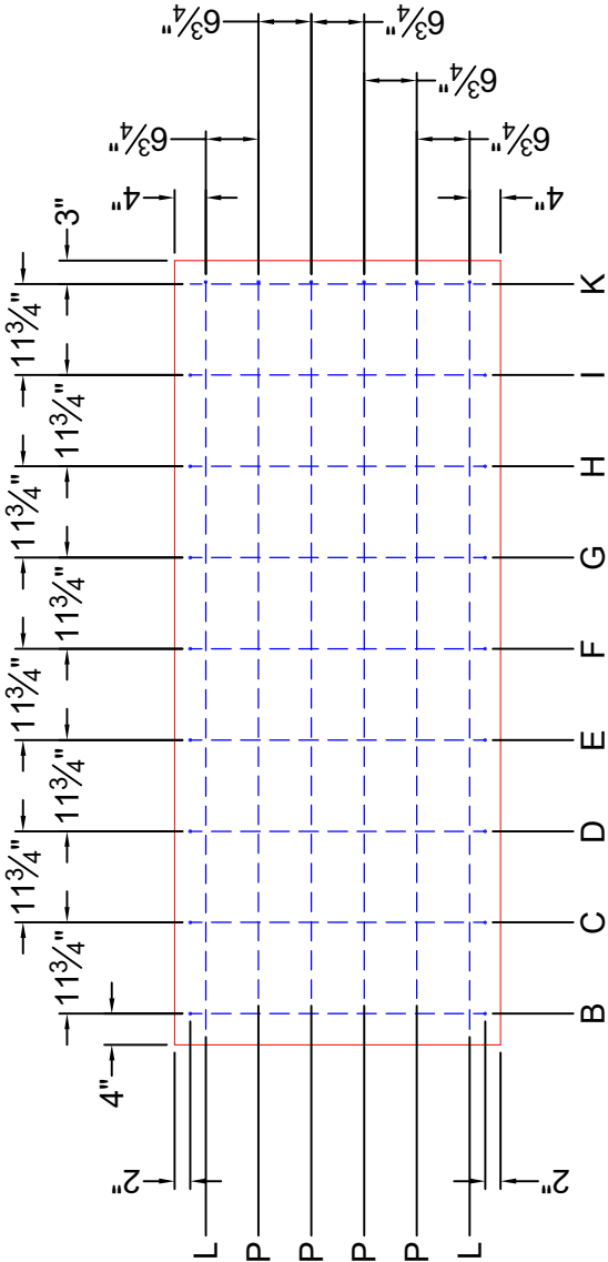
MAT REBAR LAYOUT
