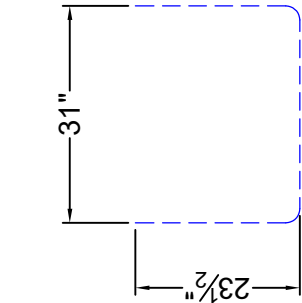
PART: D #4 REBAR GRADE 60 TOTAL LENGTH - 78" (1) REQUIRED
