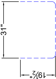
PART: E #4 REBAR GRADE 60 TOTAL LENGTH - 70" (1) REQUIRED
