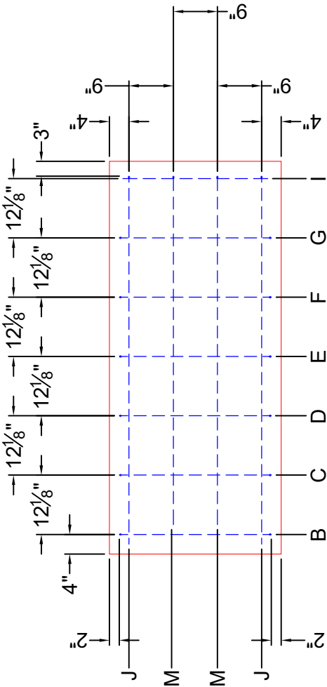
MAT REBAR LAYOUT
