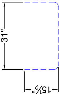
PART: F #4 REBAR GRADE 60 TOTAL LENGTH - 62" (1) REQUIRED
