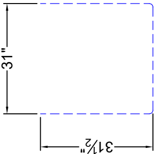
PART: B #4 REBAR GRADE 60 TOTAL LENGTH - 94" (1) REQUIRED
