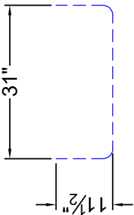
PART: G #4 REBAR GRADE 60 TOTAL LENGTH - 54" (1) REQUIRED
