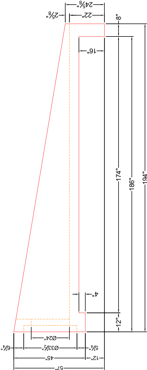
SIDE ELEVATION
