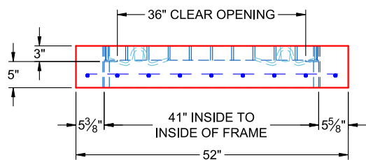
VIEW B
