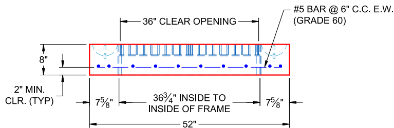
VIEW A
