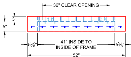
VIEW B
