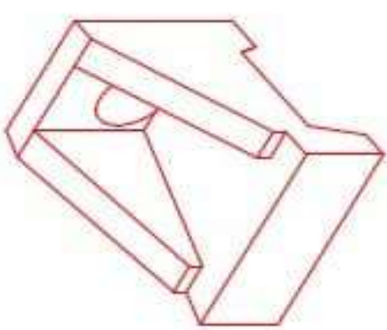
ISOMETRIC VIEW 18" HEADWALL
