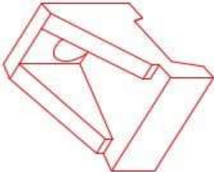
ISOMETRIC VIEW 24" HEADWALL
