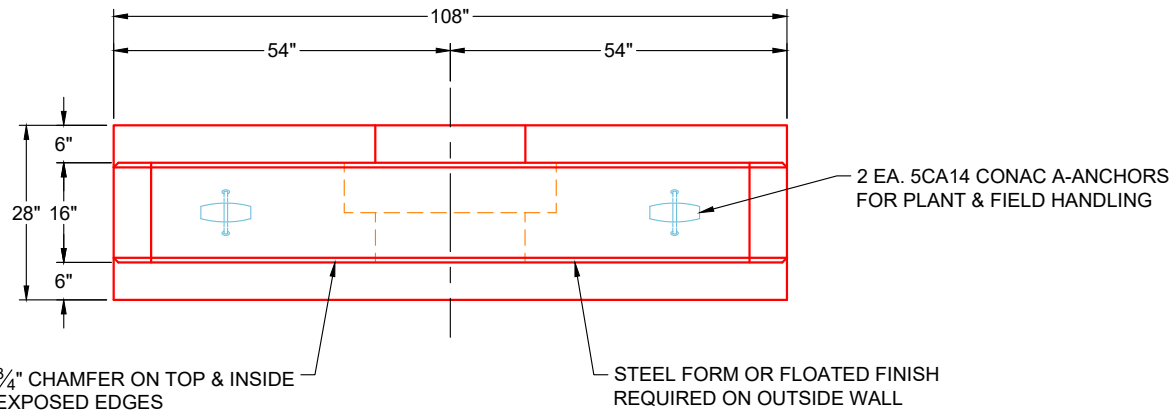
PLAN VIEW
