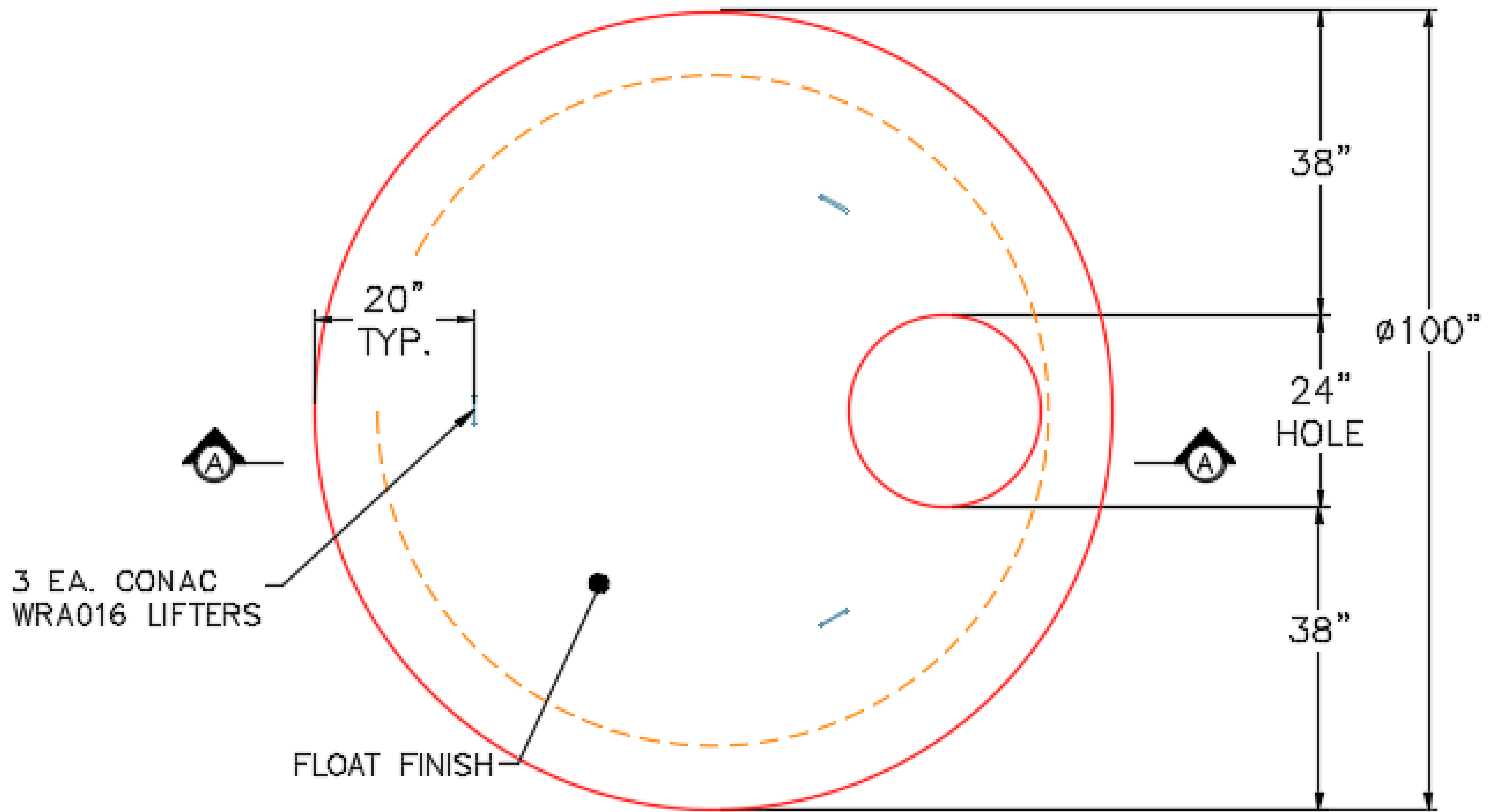
PLAN VIEW
