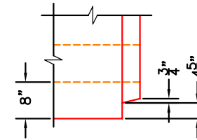
JOINT DETAIL (TYP.) NTS
