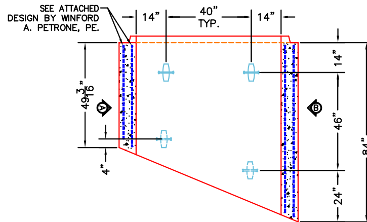
PLAN VIEW UPRIGHT IN MOLD
