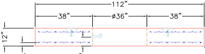
FRONT VIEW
