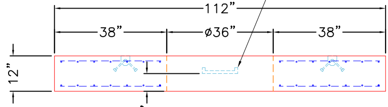
RIGHT VIEW
