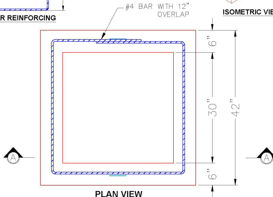
PLAN VIEW
