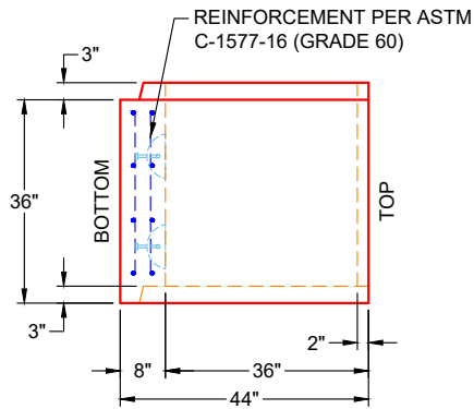
VIEW A PC 4 (UPRIGHT IN MOLD)
