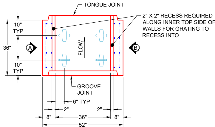
PLAN VIEW PC 4 (UPRIGHT IN MOLD)
