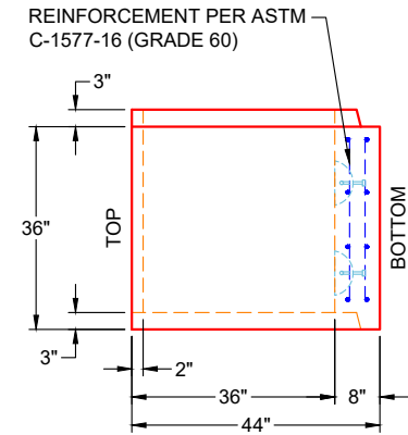
VIEW B PC 4 (UPRIGHT IN MOLD)
