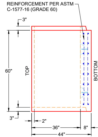
VIEW B PC 2 (UPRIGHT IN MOLD)
