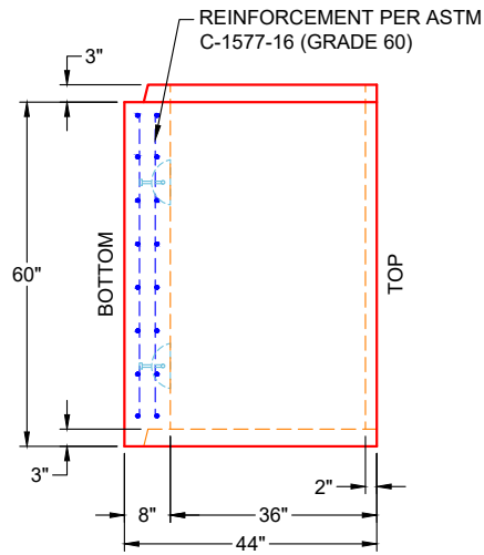
VIEW A PC 2 (UPRIGHT IN MOLD)
