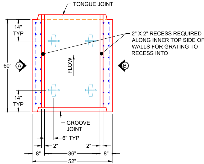
PLAN VIEW PC 2 (UPRIGHT IN MOLD)
