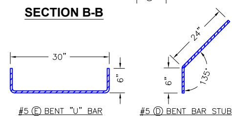
#5 (E) BENT "U" BAR
