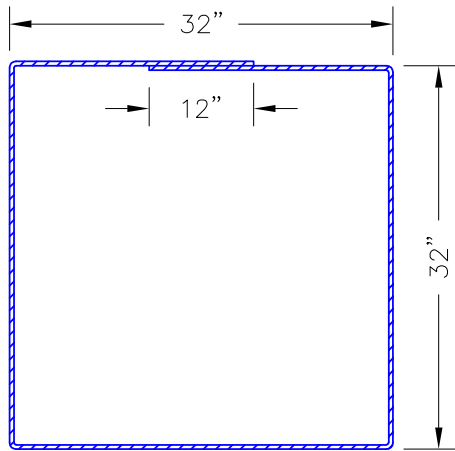
#4 BAR REINFORCING
