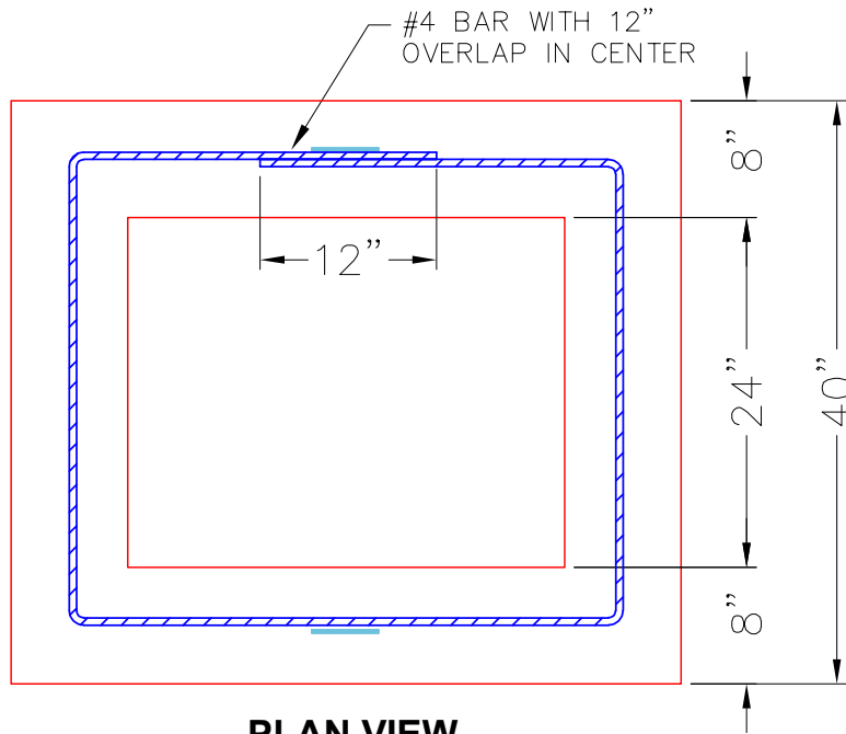
PLAN VIEW
