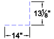
BAR - F #5 BAR (GRADE 60) TOTAL LENGTH - 27.125" (1) - TOTAL REQUIRED
