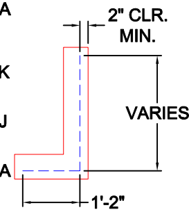
END VIEW
