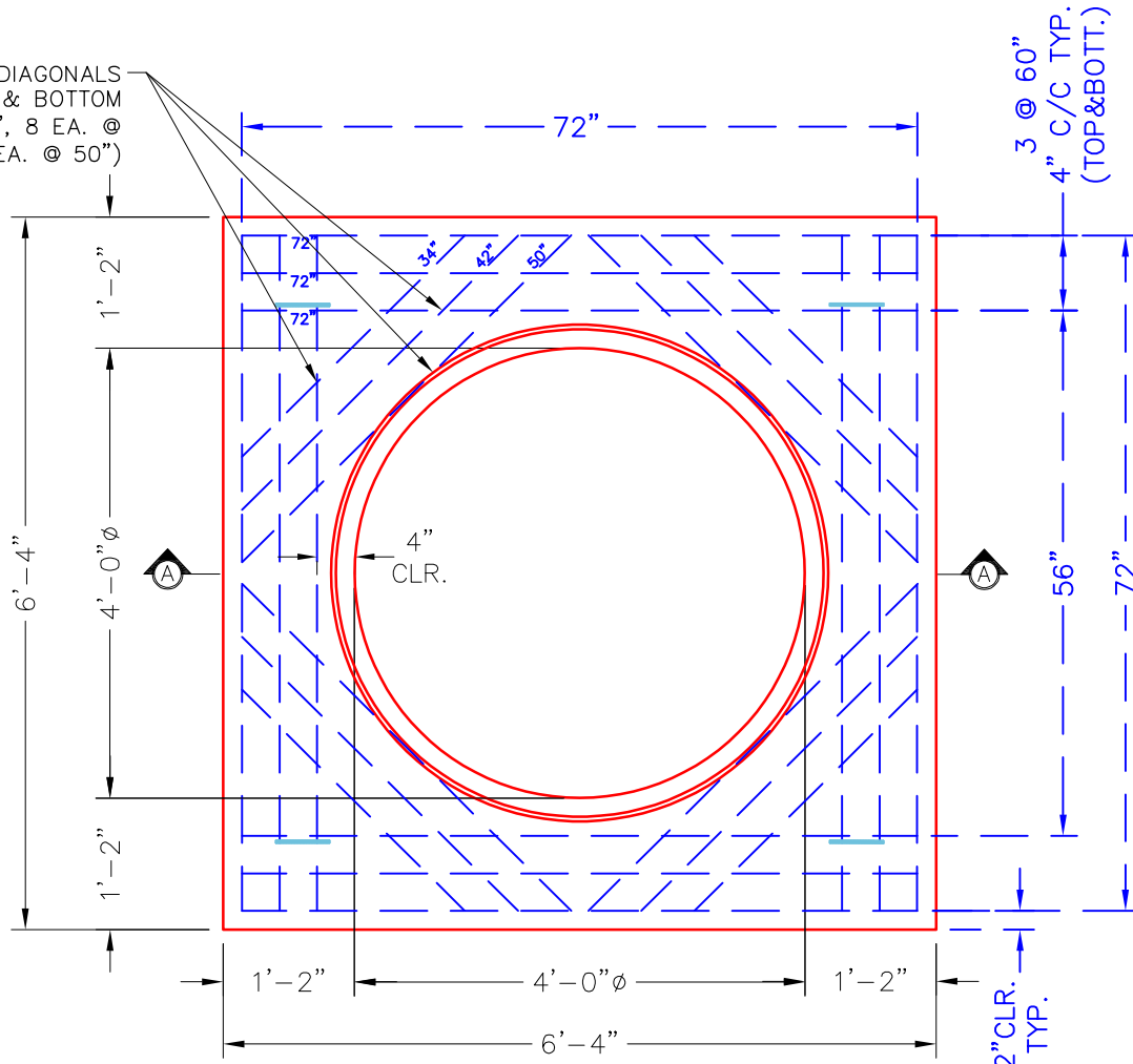
PLAN VIEW
