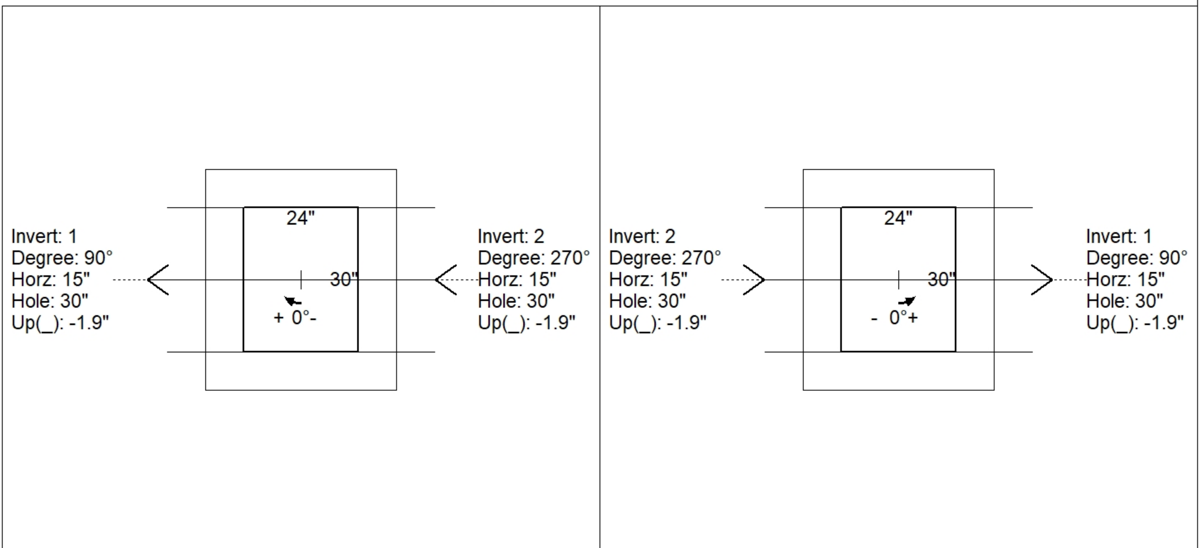
UPSIDE-DOWN VIEW (int. dimensions)
