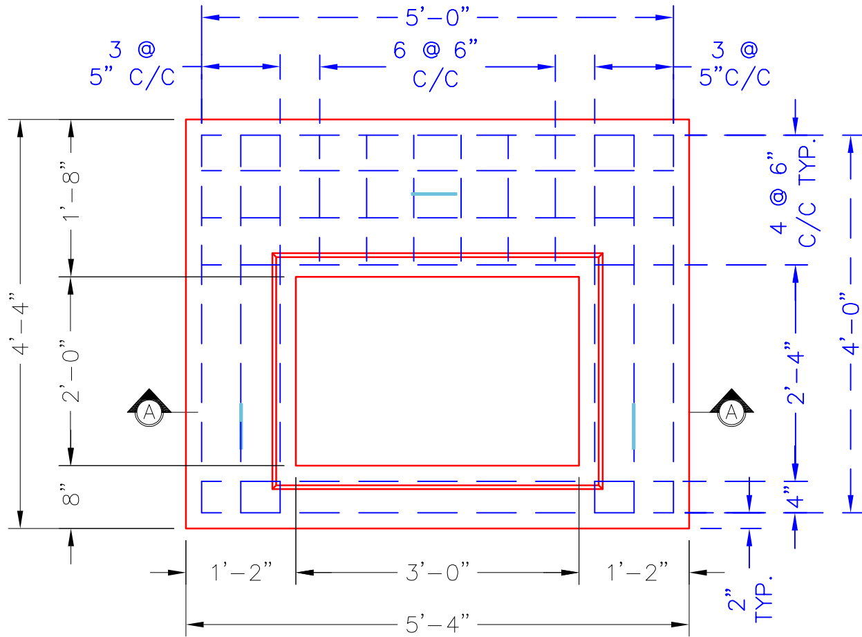
PLAN VIEW
