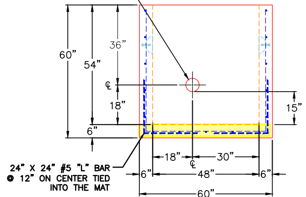
RIGHT VIEW
