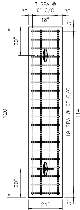
TOP VIEW
