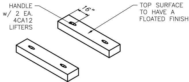
84"x18"x10" FOOTERS 2 EA.
