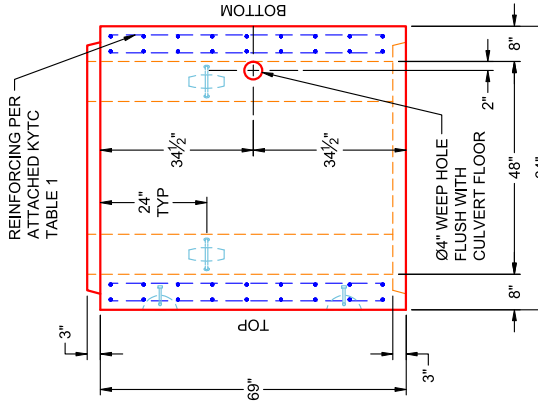
VIEW B PC 8 (UPRIGHT IN MOLD)
