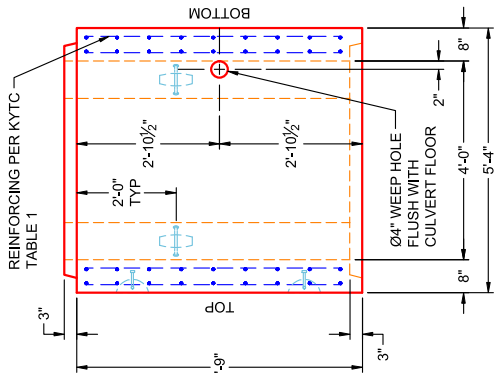
VIEW B PC 7
