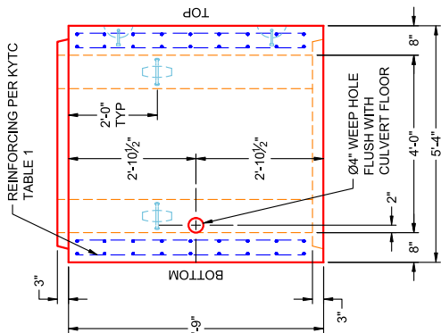
VIEW A PC 7
