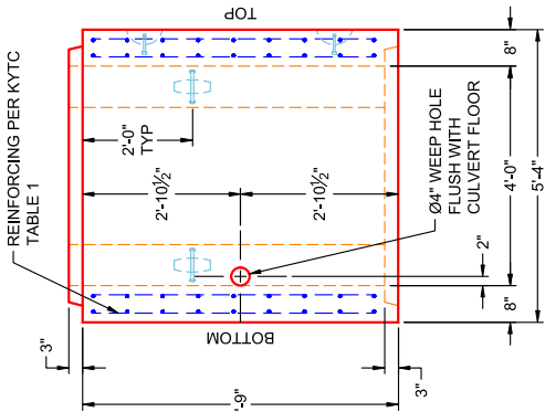
VIEW A PC 6
