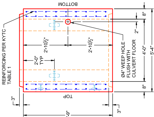
VIEW B PC 6
