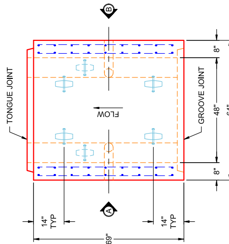
PLAN VIEW PC 6 (UPRIGHT IN MOLD)
