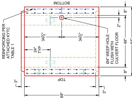
VIEW B PC 6 (UPRIGHT IN MOLD)
