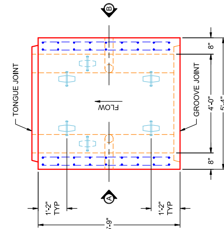
PLAN VIEW PC 5
