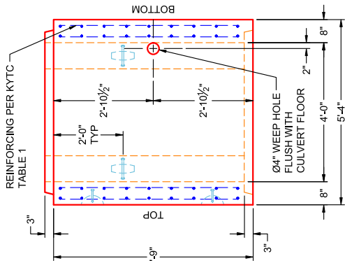
VIEW B PC 5
