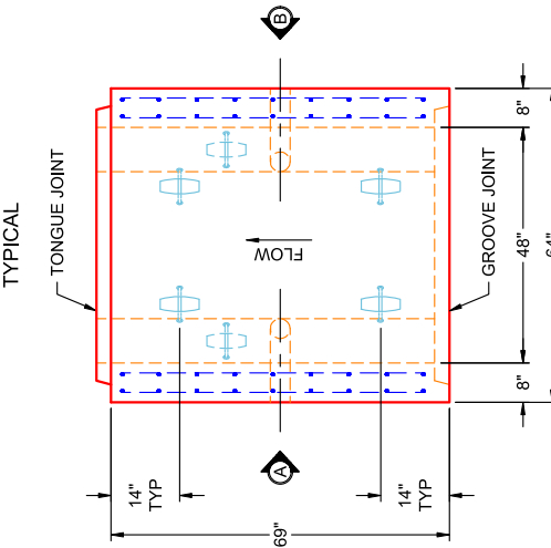
PLAN VIEW PC 4 (UPRIGHT IN MOLD)
