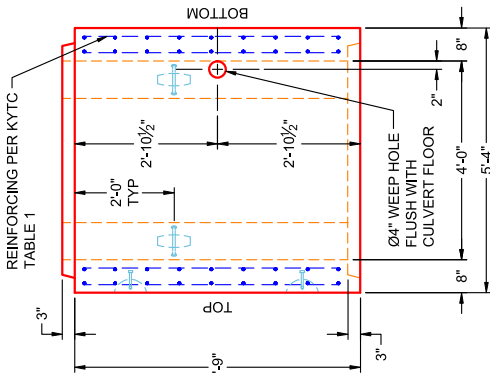
VIEW B PC 3
