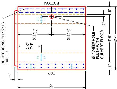
VIEW B PC 19
