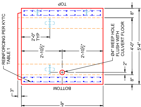
VIEW A PC 19
