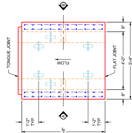
PLAN VIEW PC 19
