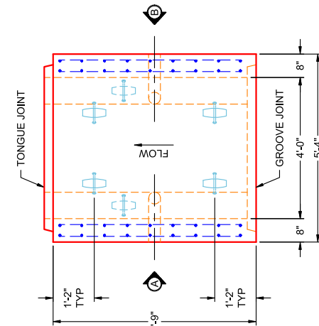
PLAN VIEW PC 17
