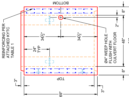
VIEW B PC 17 (UPRIGHT IN MOLD)
