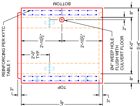
VIEW B PC 16
