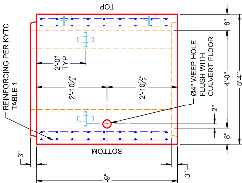
VIEW A PC 16
