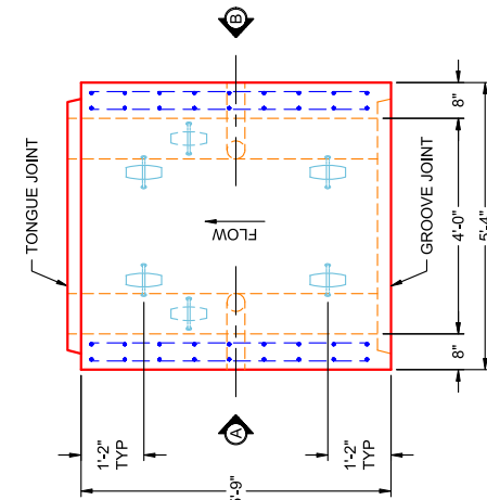
PLAN VIEW PC 16
