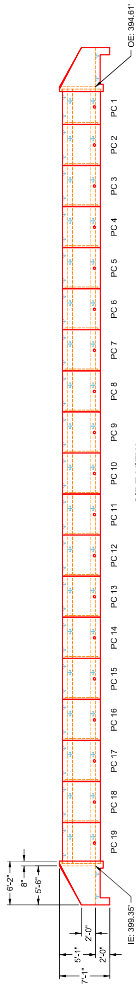
SIDE VIEW
