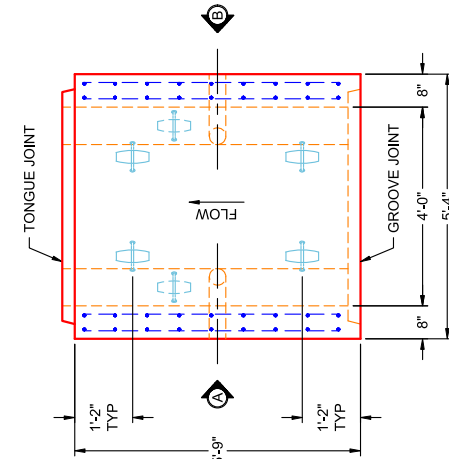
PLAN VIEW PC 15
