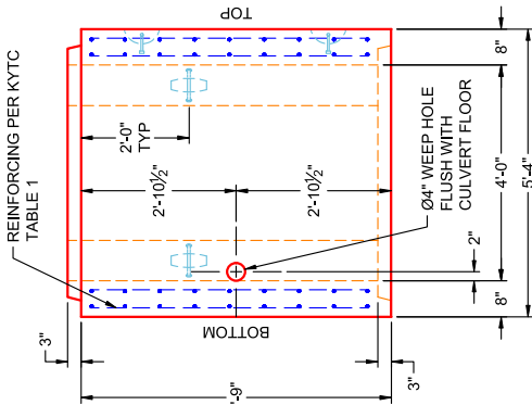
VIEW A PC 15
