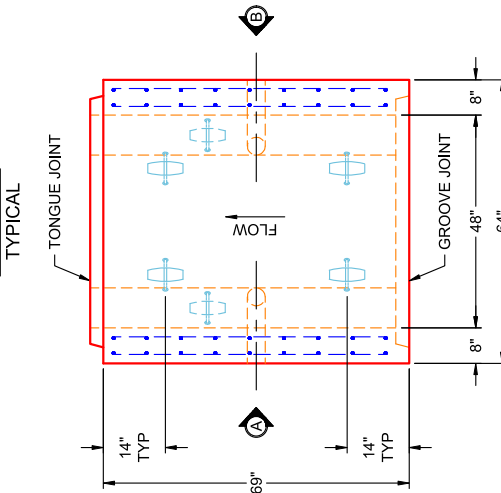
PLAN VIEW PC 13 (UPRIGHT IN MOLD)
