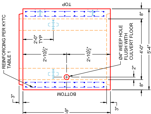
VIEW A PC 12
