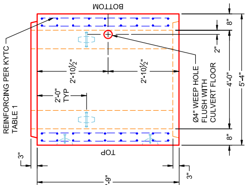
VIEW B PC 12
