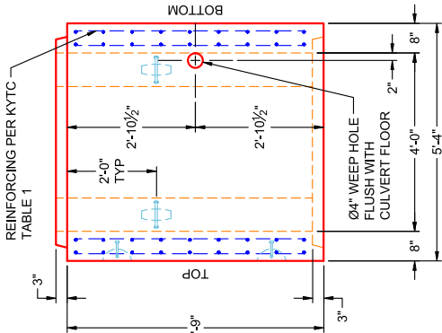
VIEW B PC 10
