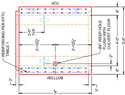
VIEW A PC 10
